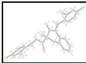
Fig. 1. The molecular structure showing 30% probability displacement ellipsoids (arbitrary spheres for H atoms).
